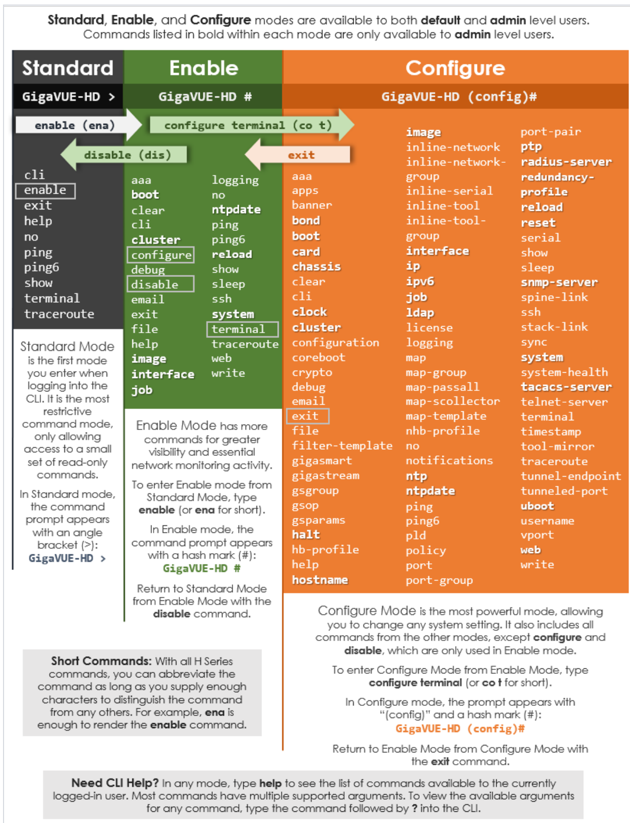
Figure 1 GigaVUE-OS Command-Line Modes Cheat Sheet
